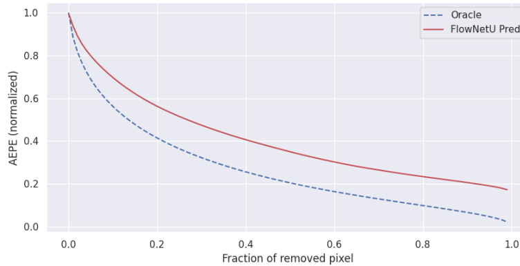
Figure 4: Sparsification plot on the clear Sintel train-set. The Oracle curve indicates the best ranking of uncertainty.
