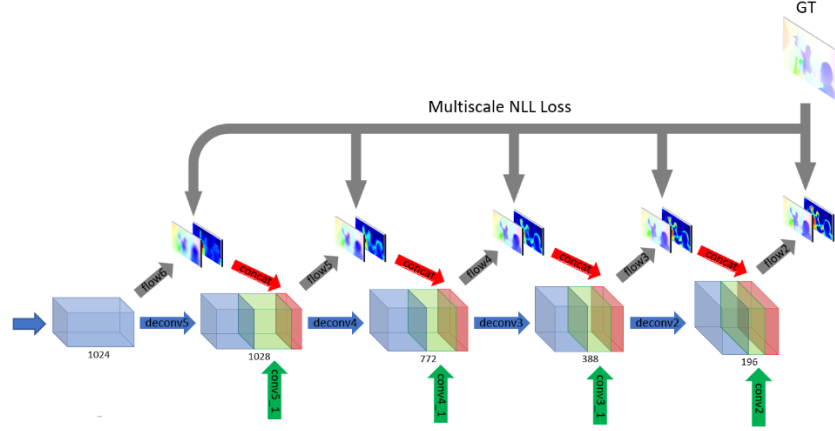
Figure 2: The decoder architecture of FlowNetU. A deconvoluted feature (blue box), a skip-connected feature from the encoder (green box) and a predicted flow field and a variance (red box) are concatenated to become the next feature. The intermediate flow fields and variances are used to calculate the multiscale NLL loss with the ground-truth. The lower resolution flow fields are assigned with lower weights.
