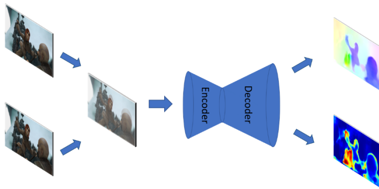
Figure 1: The encoder-decoder network of FlowNetU. FlowNetU takes a concatenation of input images as input and estimates optical flow (above) and its variance (below). The variance is used for reliable VOD.
